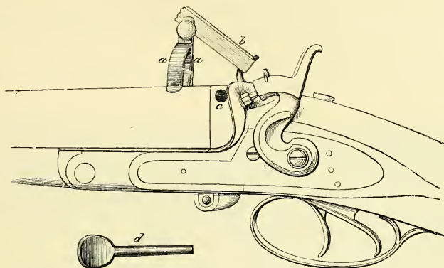
Experimental Breech-action,
